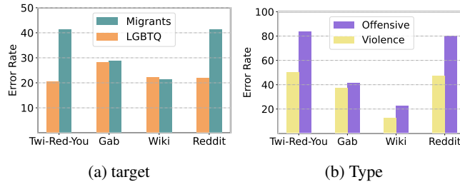
Fig. 3: Analysing error rate of PEACE under different Dimensions such as (a) hate targets (LGBTQ vs. migrants) and (b) hate type (offense vs. violence).
